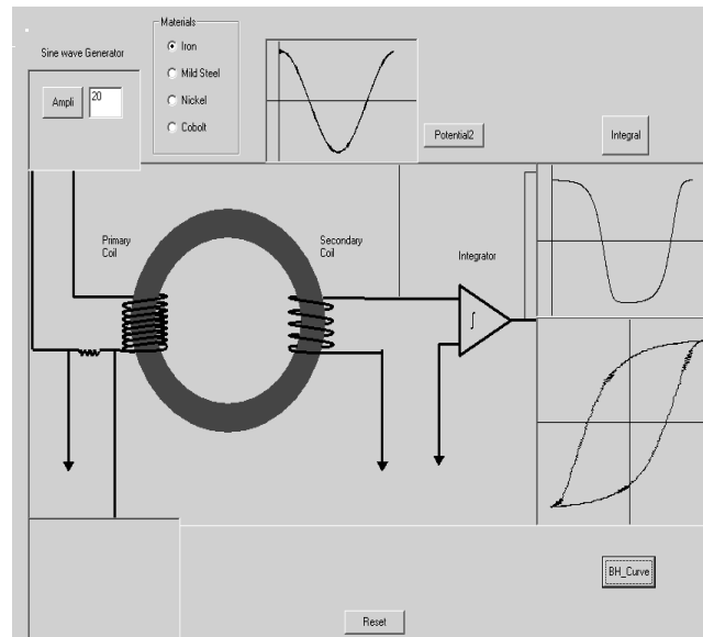
Fig. 9. Virtual experiment on ferromagnetism: B-H curve
