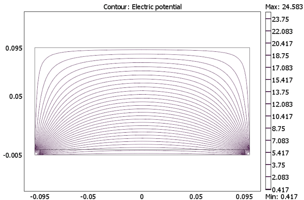
Fig. 5. Potential distribution
