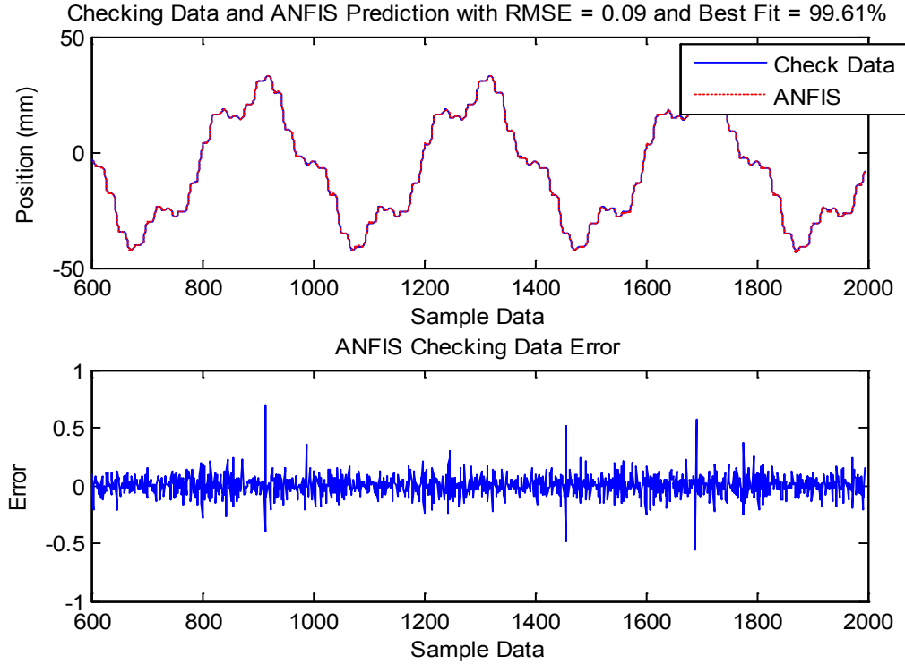
Figure 8: ANFIS 30 percent training model validation
