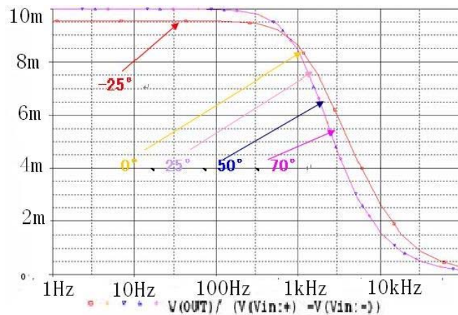
Figure 12. Simulation results under different temperatures of the voltage measurement module
