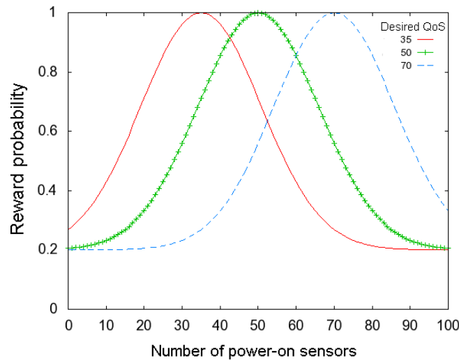
Figure 2. Reward function in the Gur Game-based scheme with K_t = 35, 50, and 70 . In a WSN, the number of active sensors contained in the sink (base) is determined by the number of received data from the active sensors. The sink broadcasts the reward value R to all sensors using the information and reward functions. The sensors can then determine whether to be active or idle in the next iteration based on the received R value from the sink. The decision is made by each sensor based on the finite-state automaton, the current state, and the received R value. The
